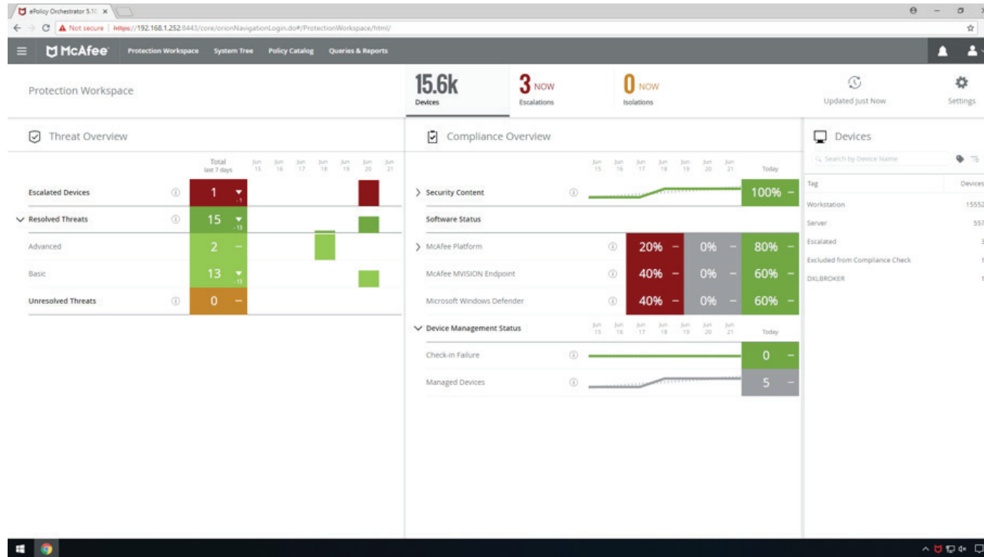
Figure 1. The McAfee ePO protection workspace.
